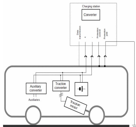
Fig. 2. Charging in four-pole system
