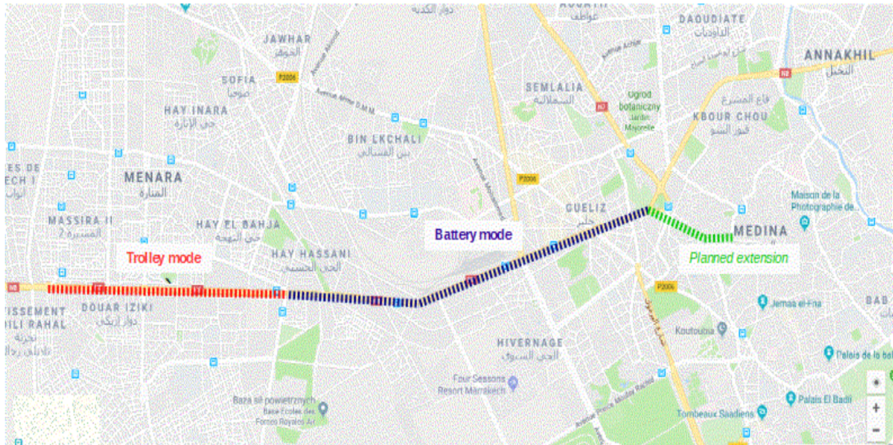
Fig. 10. The scheme of Marrakesh's BRT system
